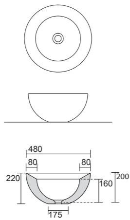
Lavabo Appoggio 200 Counter Top Washbasin 200 Ø 48 cm
