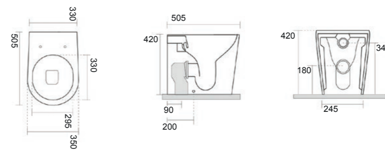
Vaso Terra BTW Wc 33x50 cm
