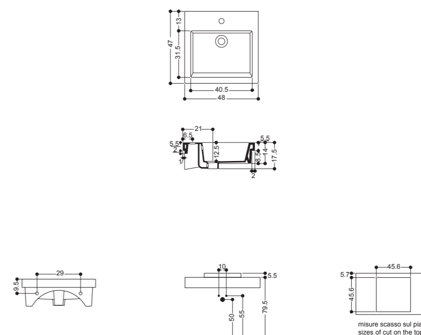
WS075 Lavabo Incasso monoforo Recessed Basin 1 hole 48x47 cm
