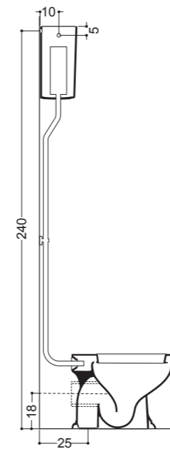
Art 06050 Cassetta Alta High level cistern 38x45,5 cm
