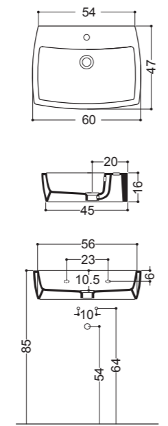
Lavabo Apoggio Overtop Basin 60x47 cm
