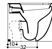
Vaso Terra BTW Wc 34x52 cm
