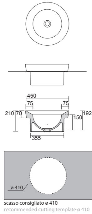
Lavabo Incasso 70 Inset Washbasin 70 Ø 45 cm
