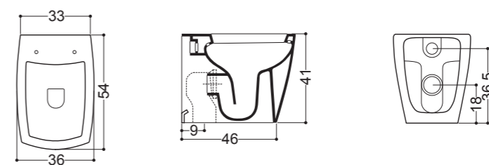
Vaso Terra BTW Wc 36x54 cm
