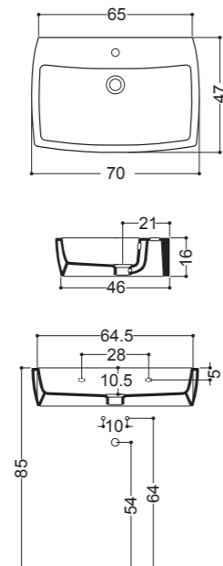
Lavabo Apoggio Overtop Basin 70x47 cm
