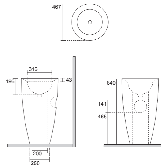
Lavabo Freestanding Parete Freestanding Washbasin Wall Ø 46 cm
