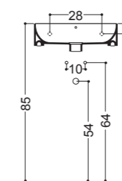
NET Lavabo NET Basin 45x35 cm
